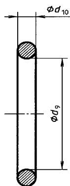
Figure 3 — O-ring
