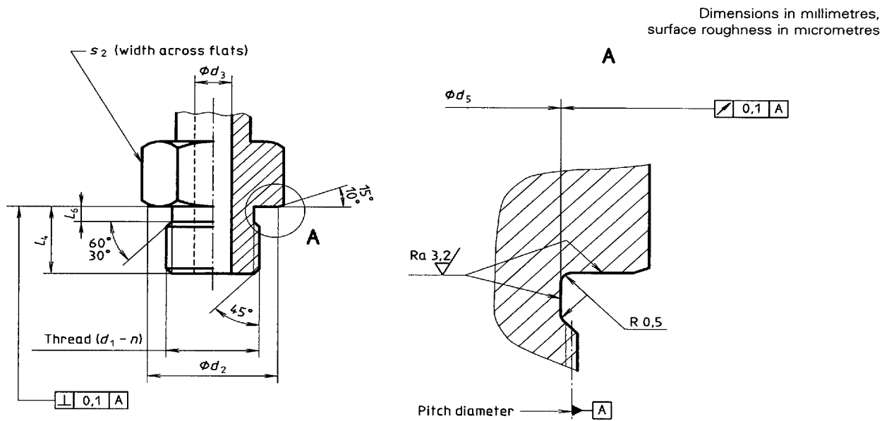
Figure 2 — Non-adjustable heavy-duty (S series) stud end
