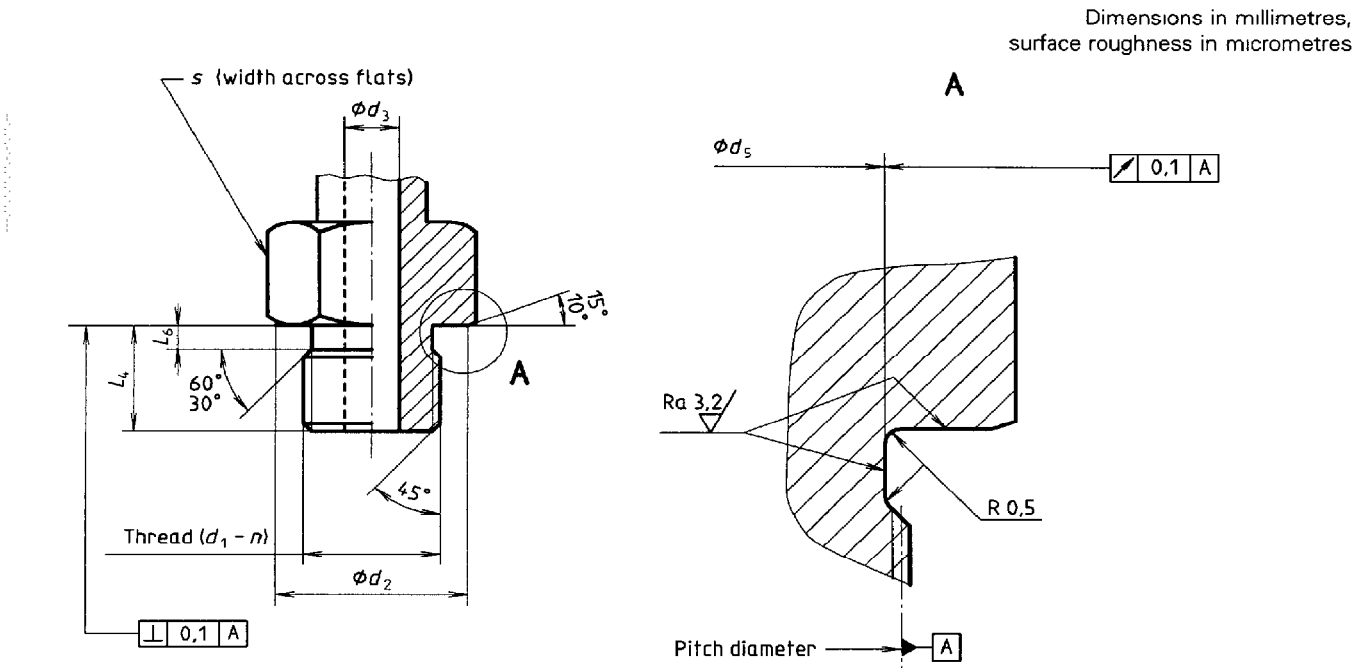
Figure 2 — Non-adjustable light-duty (L series) stud end
