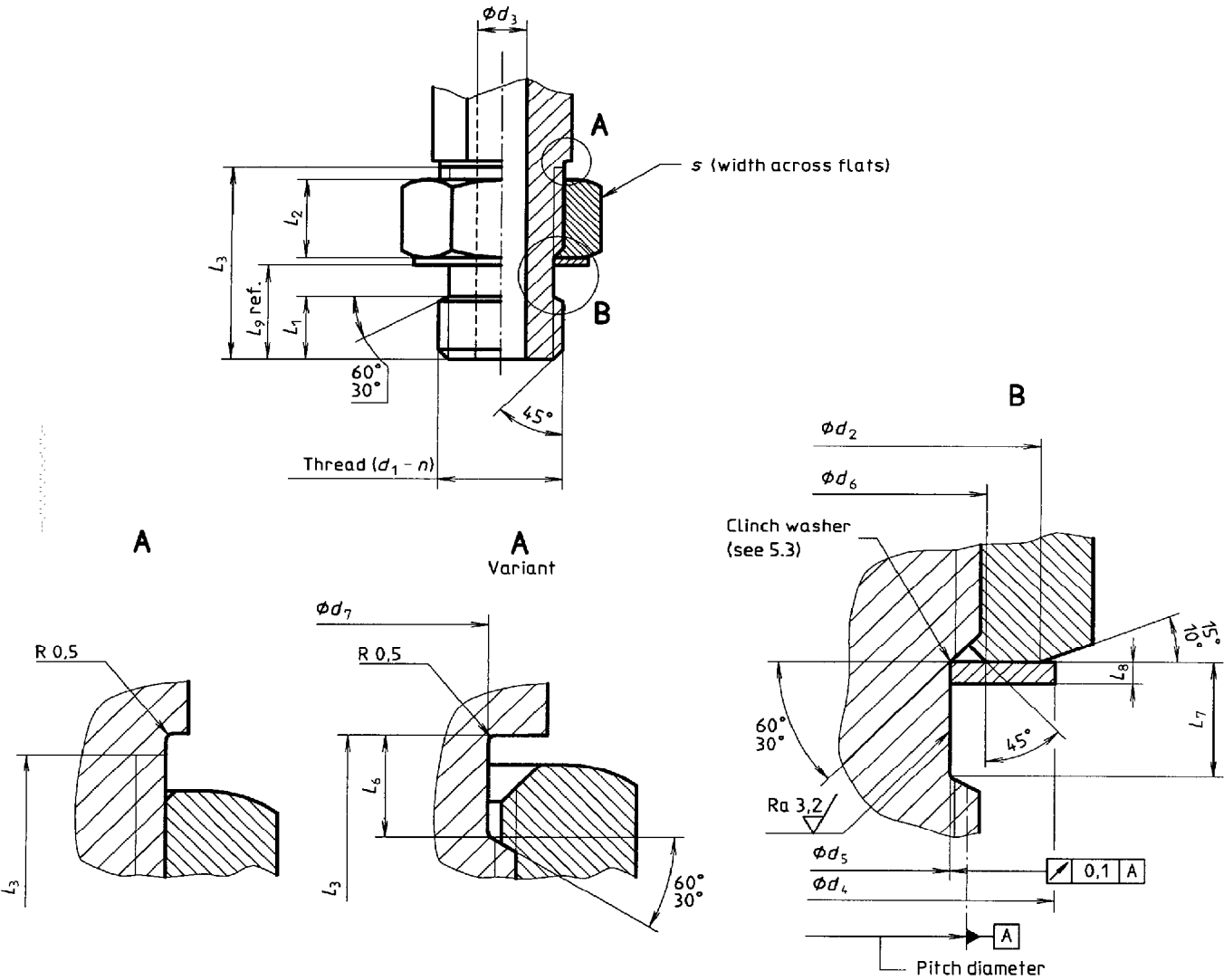
Figure 1 — Adjustable light-duty (L series) stud end
